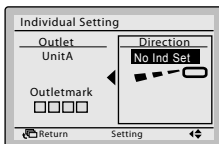
Main screen
